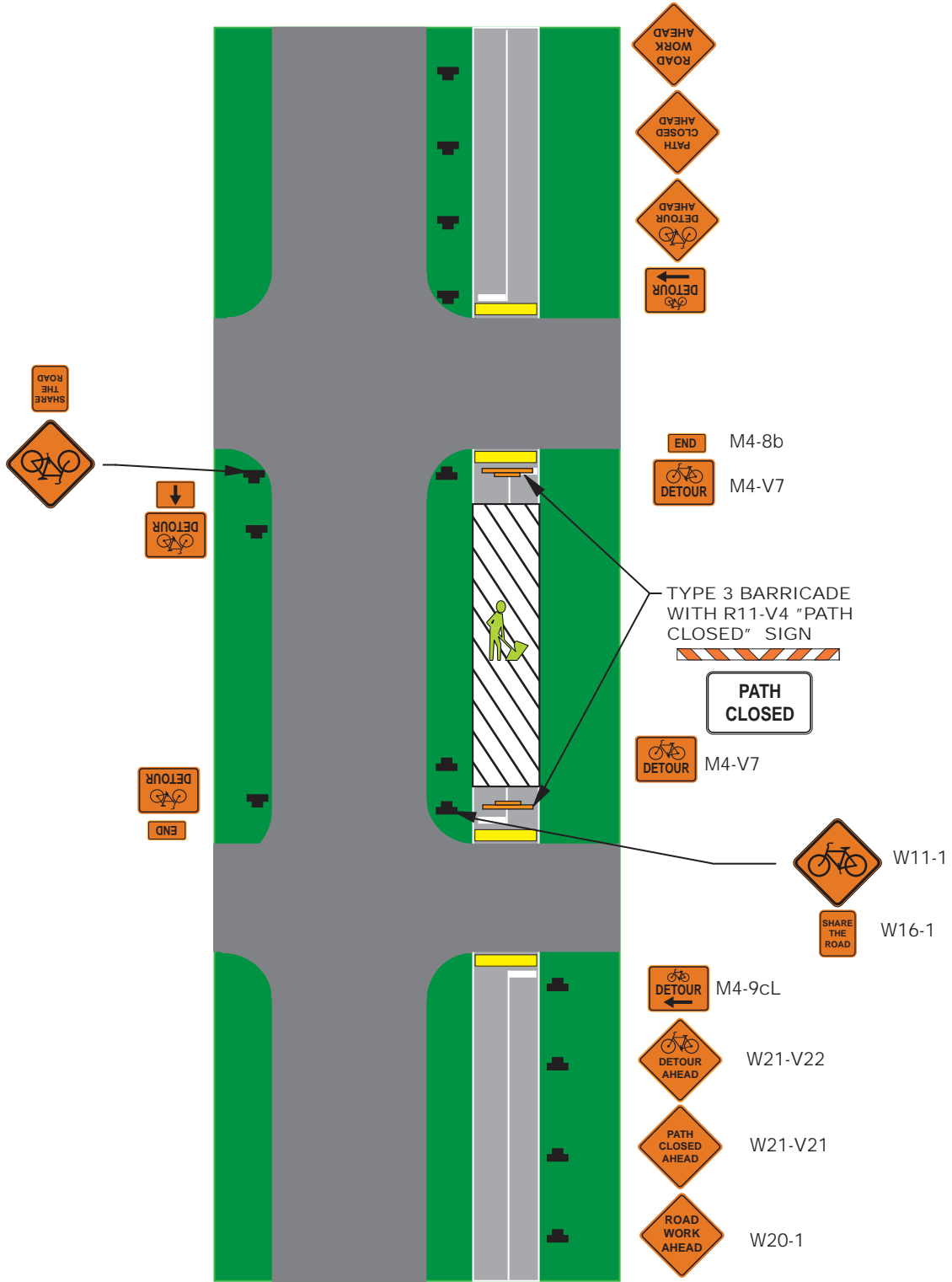
EXAMPLE OF A SHARED-USE OR BICYCLE PATH CLOSURE WITH DIVERSION
